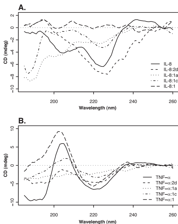
Fig. 3. (A) Interaction of heparin and derivatives in solution with IL-8 demonstrated through changes in protein secondary structure. SRCD spectra (185–260 nm) of IL-8 in the presence of selected test compounds ( 1a , 1c , 2d ), unmodified porcine mucosal heparin ( 1 ) and the natural ligand heparan sulfate (HS) in a 1:1 molar ratio. The spectra of heparin and derivatives alone were subtracted. (B) SRCD spectra (185–260 nm) of TNF- \alpha in the presence of heparin derivatives 1a , 1c , 2d and unmodified porcine mucosal heparin 1 , which induces changes in the secondary structure of the protein, demonstrating a direct interaction in solution.
