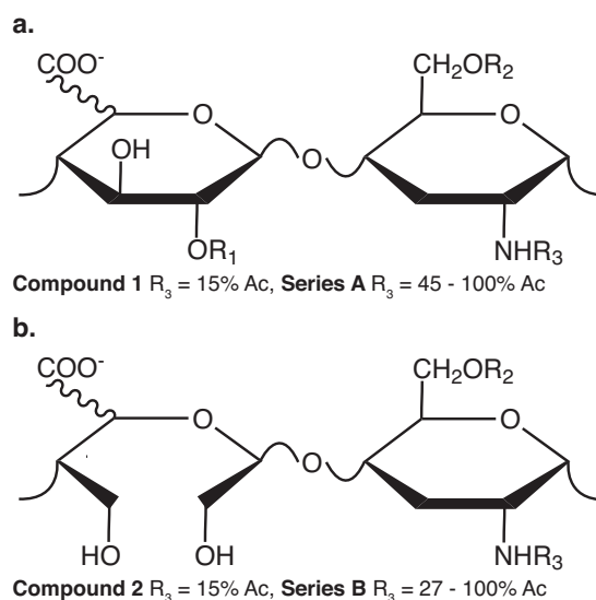
Scheme 1. (A) The repeating disaccharide unit of the compounds comprising series A and B, based on R_1 and R_2 = \text{H}/\text{SO}_3^- , R_3 = \text{SO}_3^-/\text{COCH}_3 . The uronic acid in these compounds (derived from PMH) is predominantly in the form L-iduronic acid (L-IdoA and L-IdoA-2-O-sulfate; \sim 80\% ) with D-glucuronic acid (D-GlcA; \sim 20\% ) making up the remainder. (B) Series B contains the glycol-split uronic acid residue (see Table 1 for full details of series A and B compounds).
