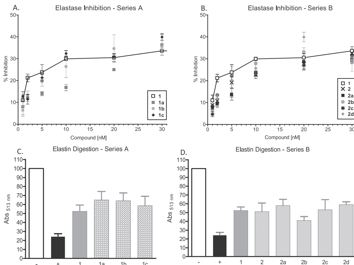
Fig. 1. Inhibition of human leukocyte elastase by heparin derivatives in assays measuring release of \rho -nitroaniline from a chromogenic peptide substrate, (A) (1a–1c) and (B) (2a–2d). The increase in absorbance at 513 nm reports the inhibition of digestion of the natural substrate ( \alpha -elastin), (C) (compounds 1, 1a–1c) and (D) (compounds 2, 2a–2d). The negative control is the level of digestion in the presence of inactive enzyme, while the positive control is the digestion in the absence of inhibitors. Results shown are averages of 3 independent experiments, each with 2 replicates, \pm standard errors. Error bars on the negative controls are negligible.
