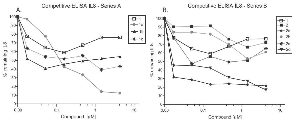
Fig. 2. Competitive ELISA showing displacement of bound IL-8 from surface immobilised heparin by 1a–1c (A) and 2a–2d (B). Reference heparin 1 is shown on both graphs.
